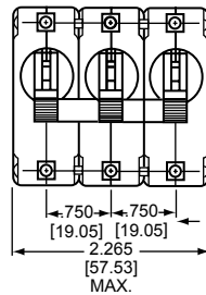
Three Pole
